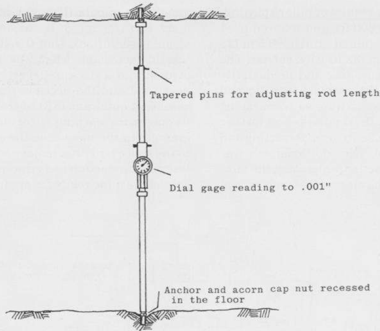
Fig. 3. "Reed" type convergence rod.
