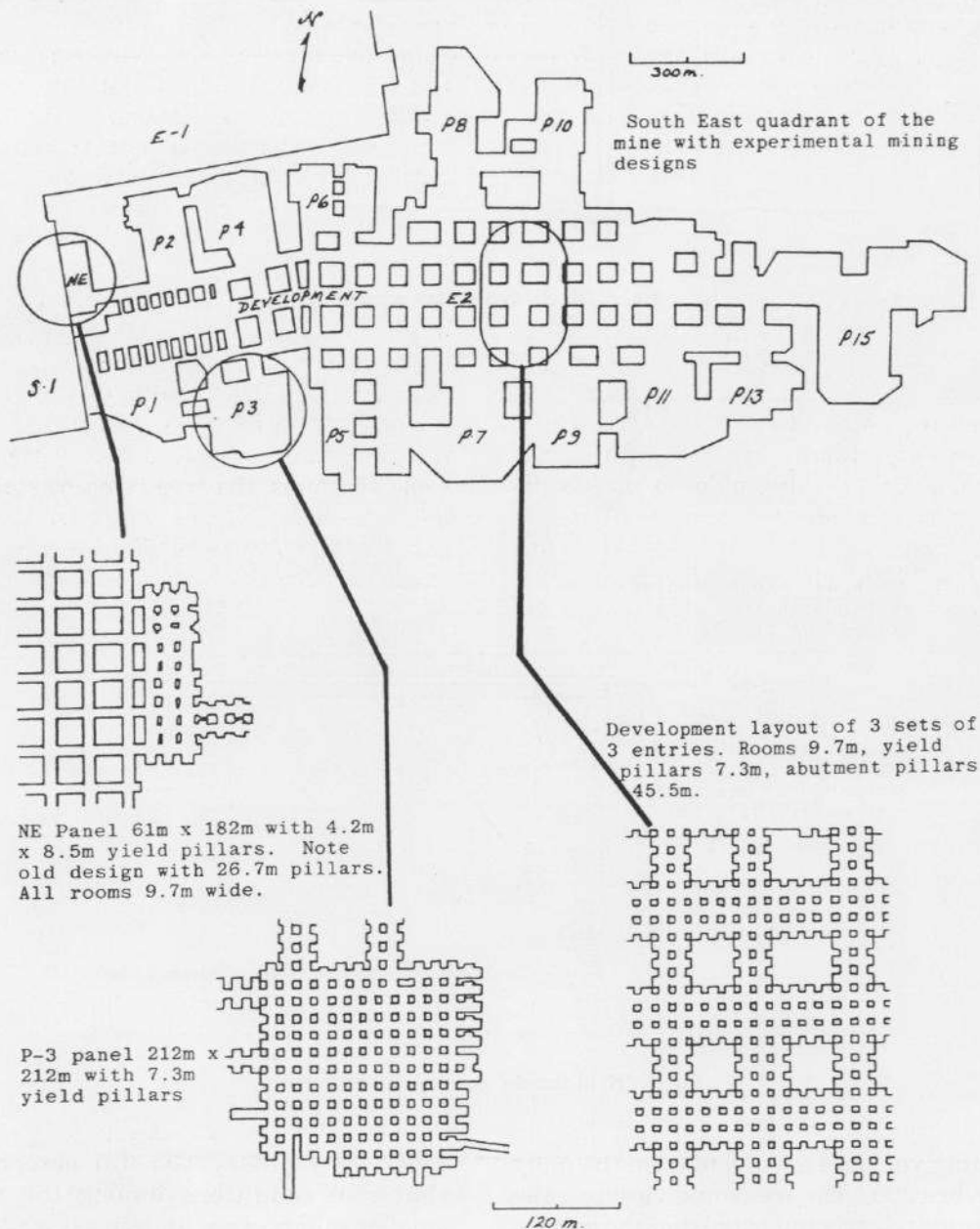
Fig. 5. Map showing south-east quadrant of the Cayuga Mine.
