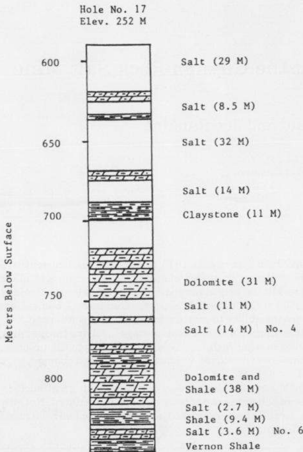
Fig. 1. Partial geologic section showing location of No. 4 and No. 6 salt beds.
