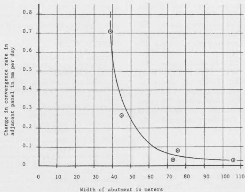
Fig. 6. Influence across abutment pillars.
