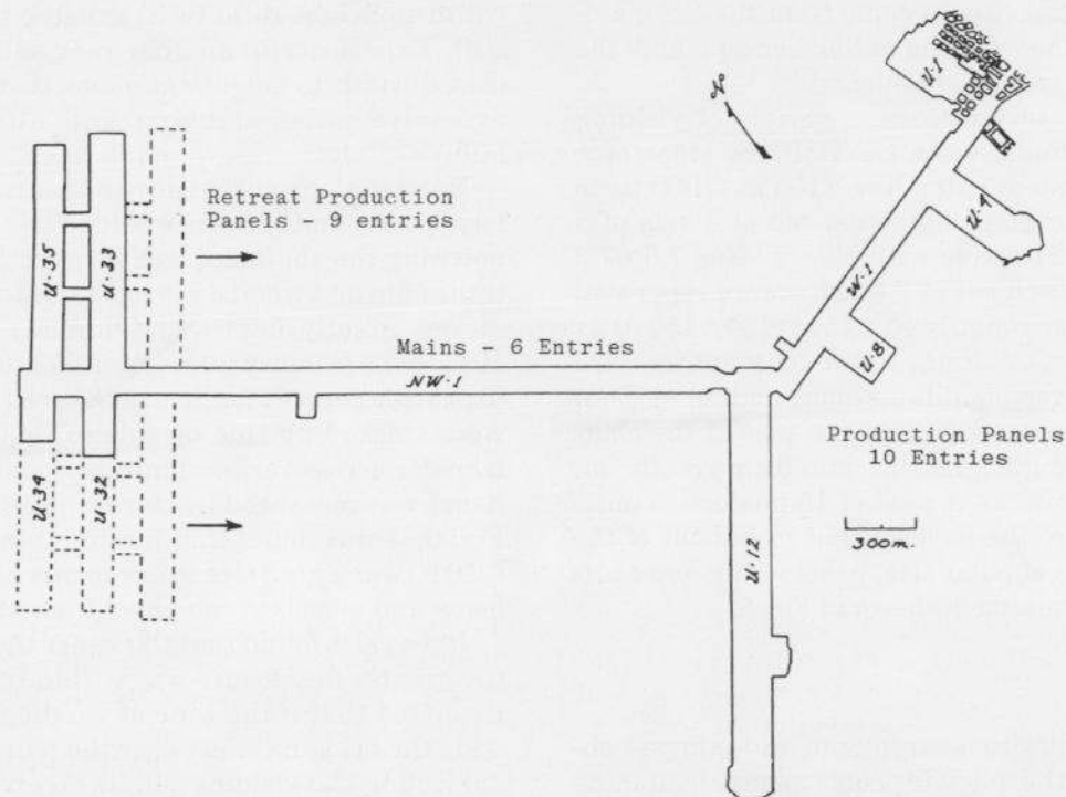
Fig. 7. North-west quadrant mining.
