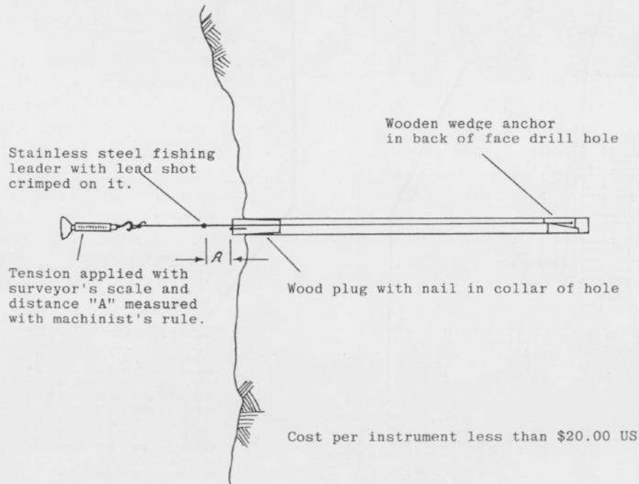
Fig. 4. "Home made" borehole extensometer.
